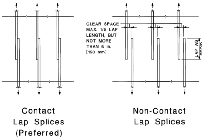
Figure 1 — Contact and non-contact tension lap splices
