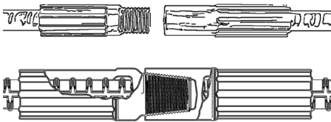
Figure 3 — Cold-swaged threaded coupler
