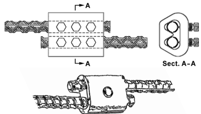
Figure 5 — Mechanical lap coupling sleeves
